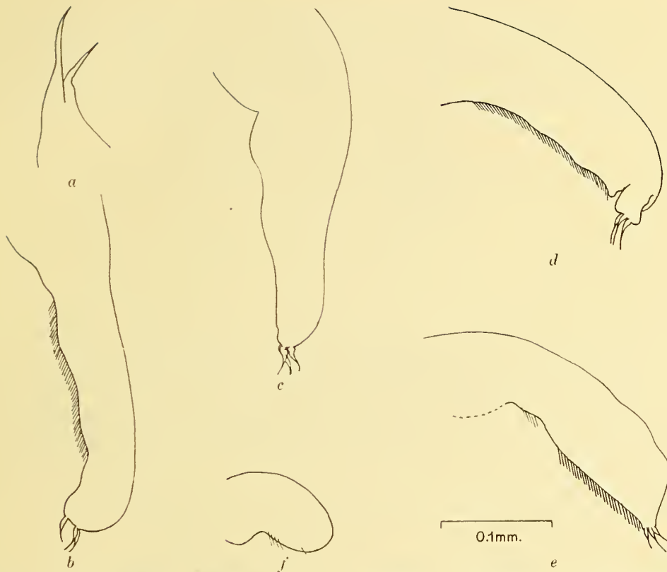
TEXT-FIG. 13.— Baccalaurus verrucosus sp. nov. Thoracic appendages. a , First thoracic appendage. b , Second thoracic appendage. c , Third thoracic appendage. d , Fourth thoracic appendage. e , Fifth thoracic appendage. f , Sixth thoracic appendage.
